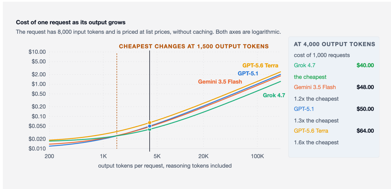
Figure 3: Each curve is one model. A curve is flat on the left, where the input cost dominates, and rises on the right, where the output cost does. Shown: output tokens per request: 4,000; input tokens per request: 8,000.
