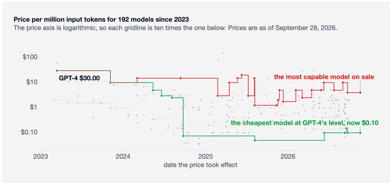
Figure 1: Each dot is one published price, and a short step joins a model’s old price to its new one where it was repriced. The two lines are one line until March 2024, when Claude 3 Opus took the top score at $15.00, and they end 40x apart. The upper line dips wherever a cheaper model held the top score, and 18 of the 23 models that have held it have estimated scores. Shown: compare providers: Whole market; class: All; price of: Input tokens.
