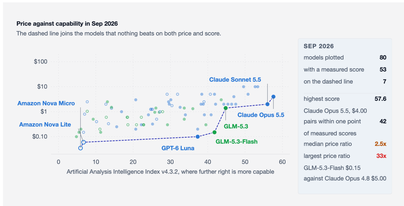
Figure 2: Each point is a model on sale, placed by its index score and its input price. A filled point has a measured score and a ring has an estimated one. Green points are open-weight models, whose weights can be downloaded, and blue points are models sold only through an API. Shown: as of: Sep 2026.
