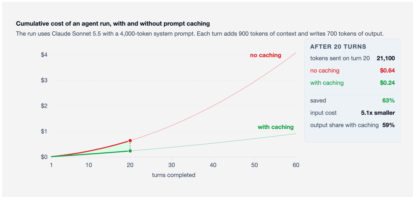
Figure 4: The solid part of each line is what the run has cost so far, and the faint part is where it is heading. Caching costs less from turn 2 on. Shown: turns completed: 20.
